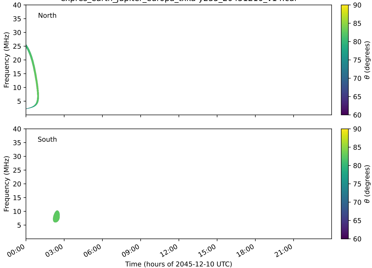
expres_earth_jupiter_europa_txka-y235_20451210_v14.cdf
