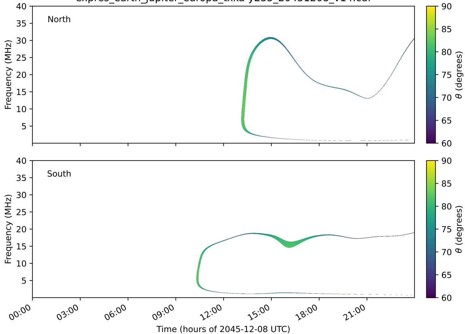
expres_earth_jupiter_europa_txka-y235_20451208_v14.cdf
