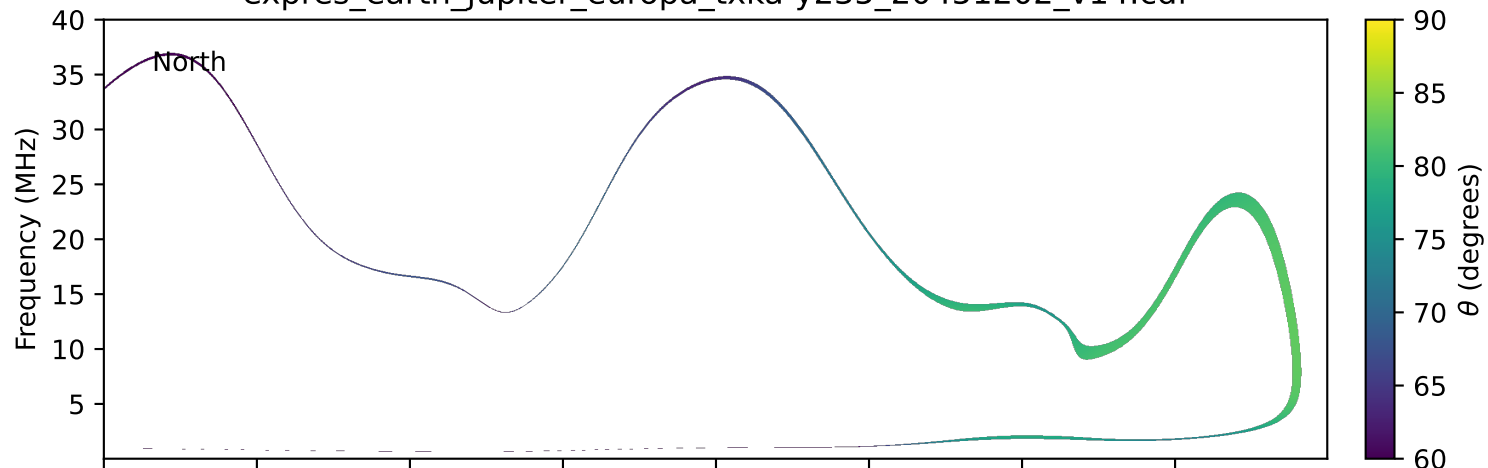
expres_earth_jupiter_europa_txka-y235_20451202_v14.cdf
