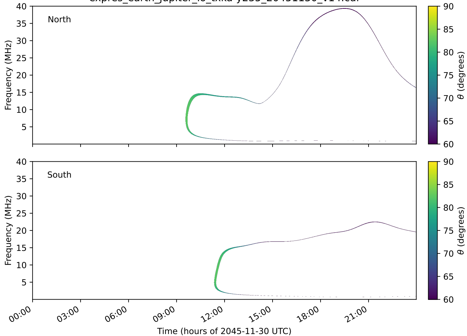
expres_earth_jupiter_io_txka-y235_20451130_v14.cdf
