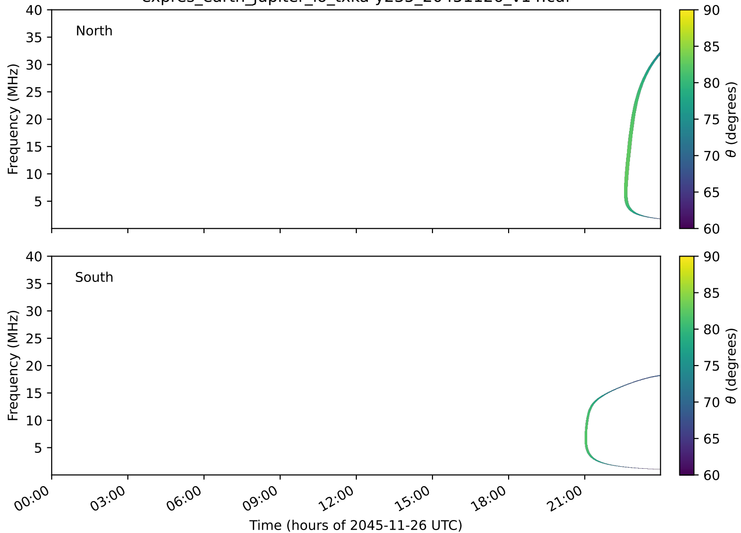
expres_earth_jupiter_io_txka-y235_20451126_v14.cdf
