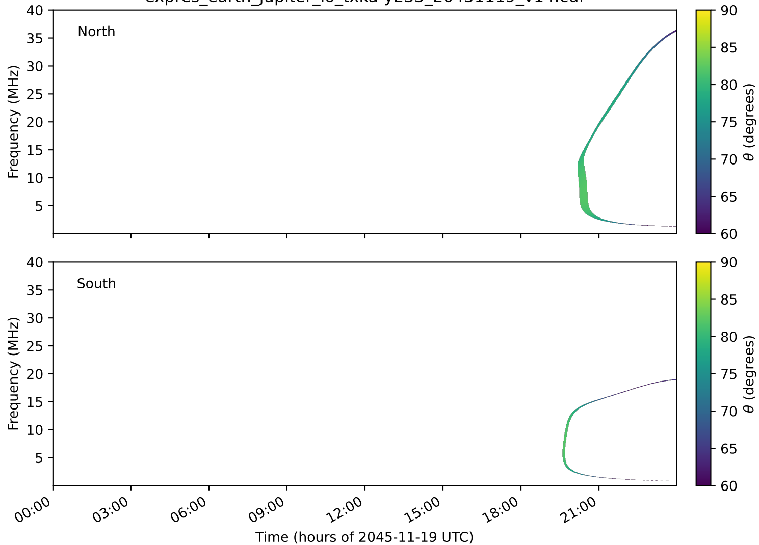
expres_earth_jupiter_io_txka-y235_20451119_v14.cdf
