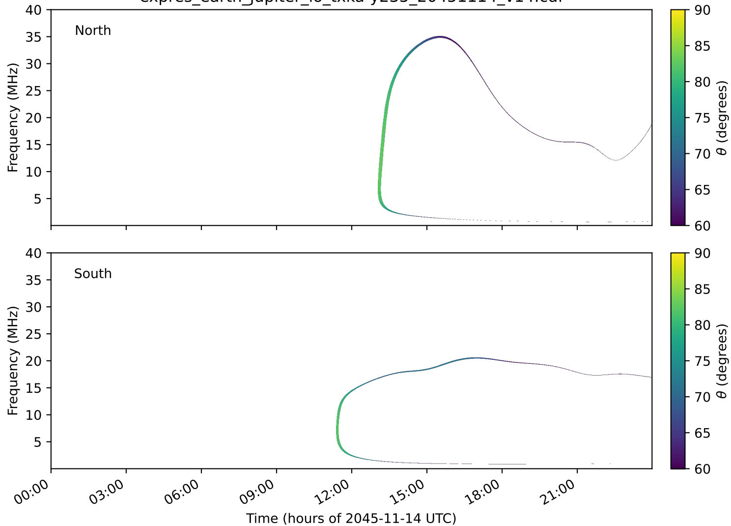
expres_earth_jupiter_io_txka-y235_20451114_v14.cdf
