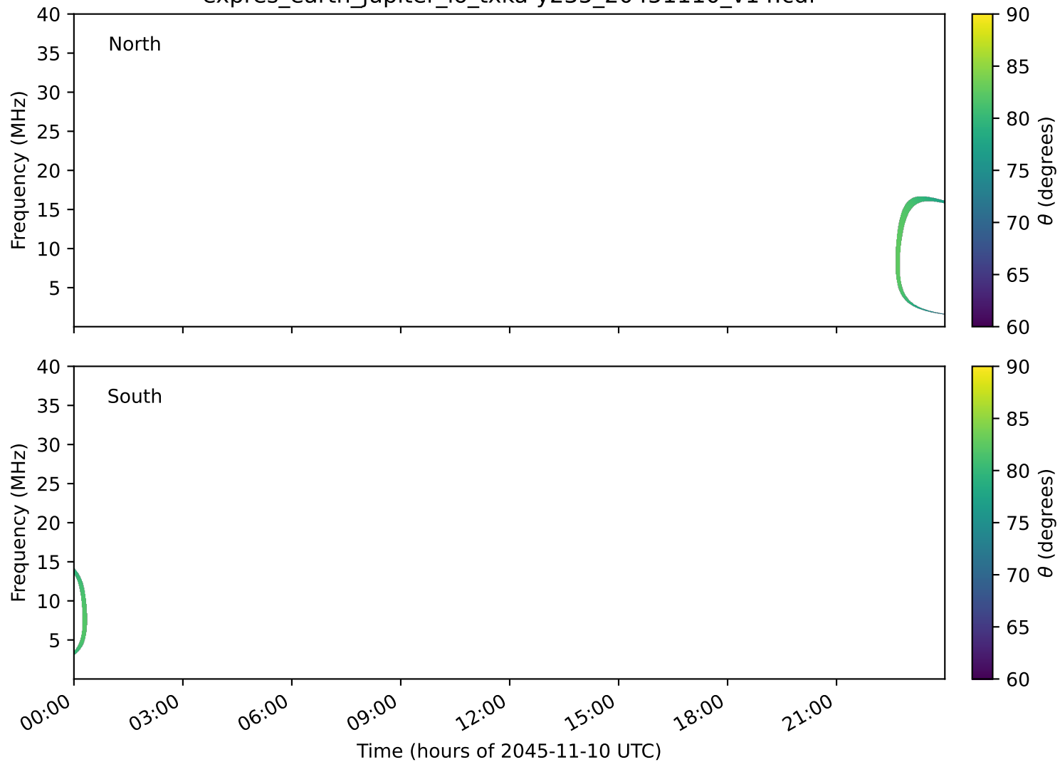
expres_earth_jupiter_io_txka-y235_20451110_v14.cdf
