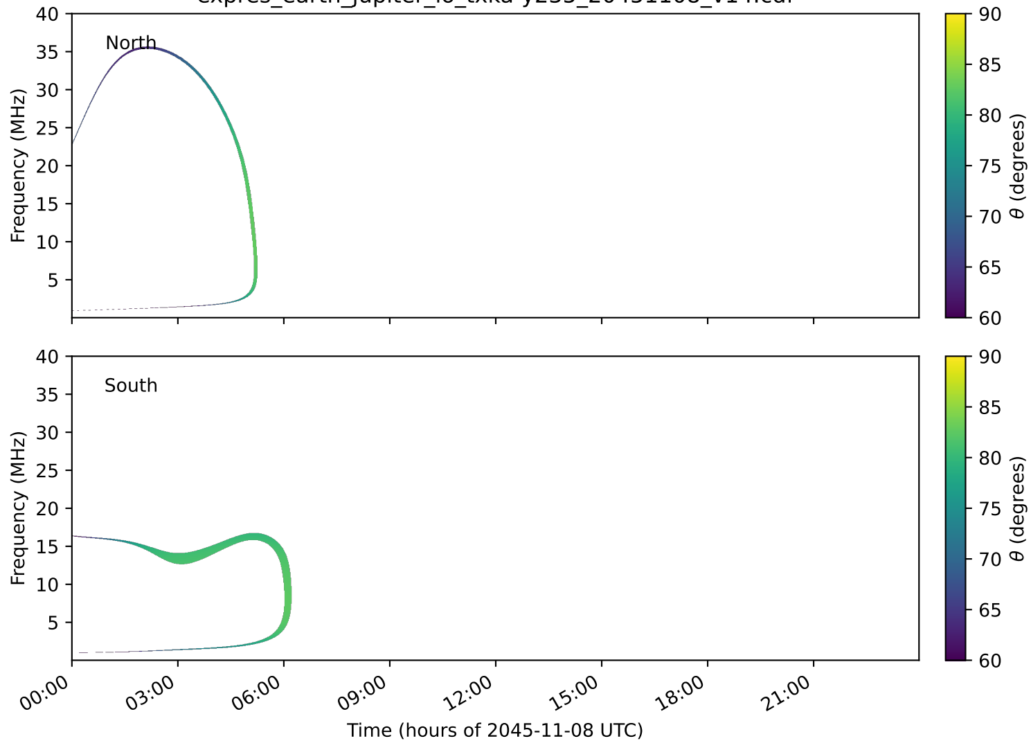
expres_earth_jupiter_io_txka-y235_20451108_v14.cdf
