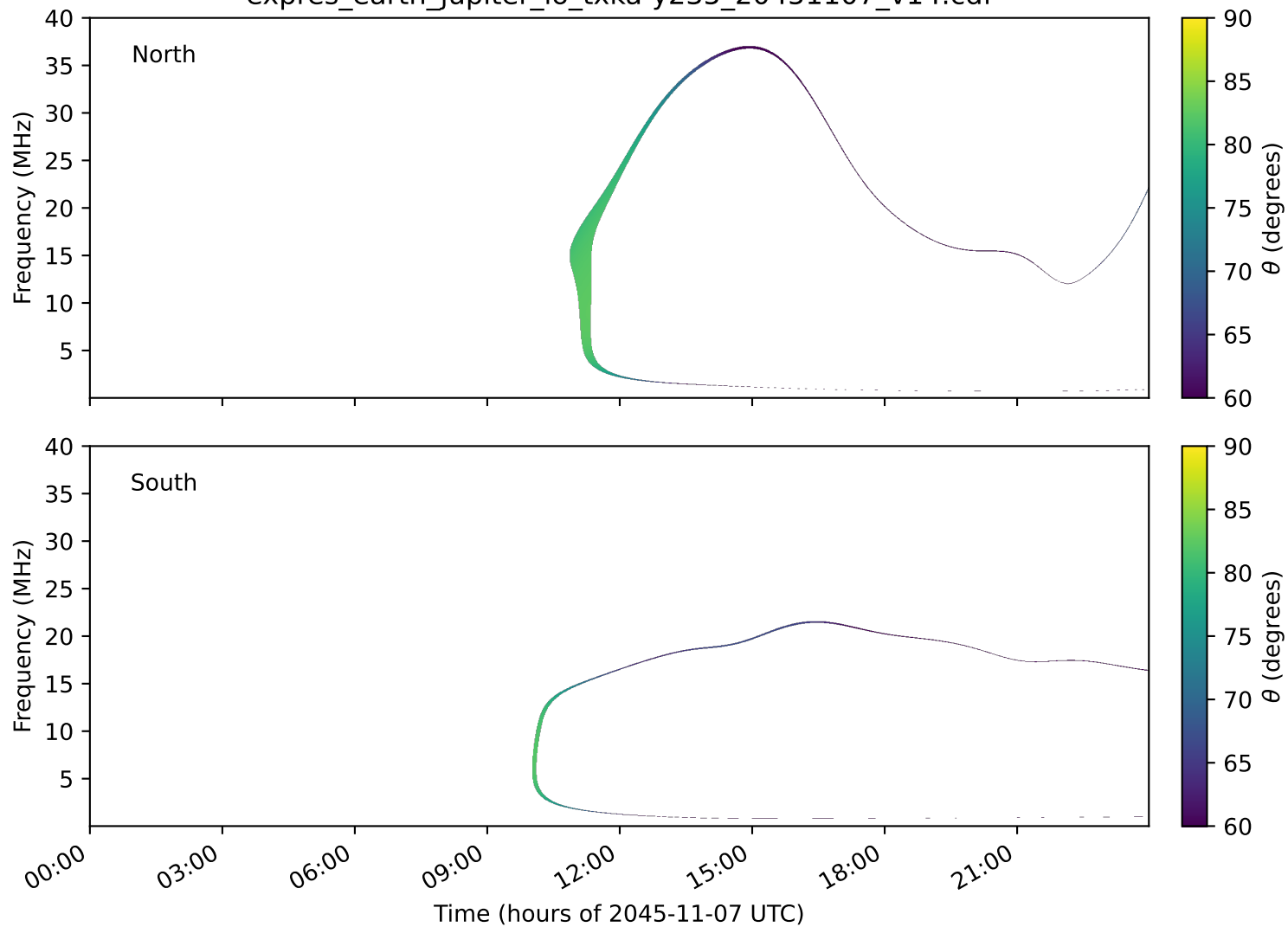
expres_earth_jupiter_io_txka-y235_20451107_v14.cdf
