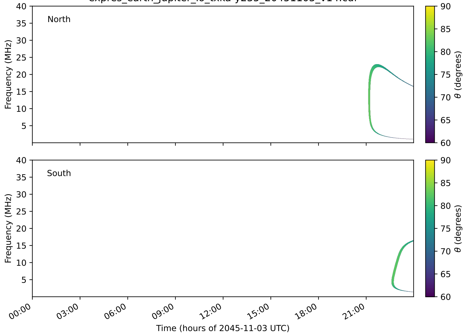
expres_earth_jupiter_io_txka-y235_20451103_v14.cdf
