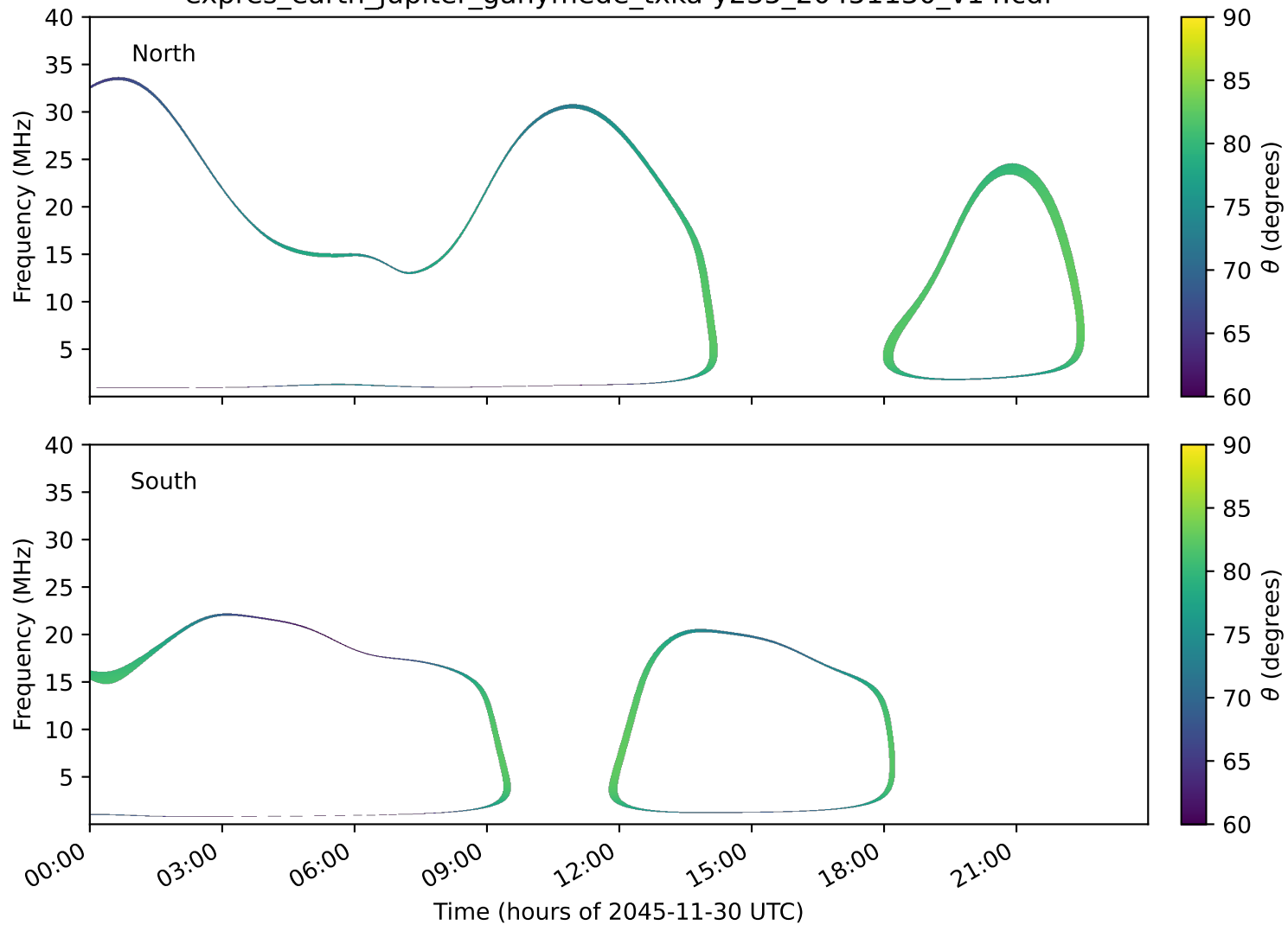
expres_earth_jupiter_ganymede_txka-y235_20451130_v14.cdf
