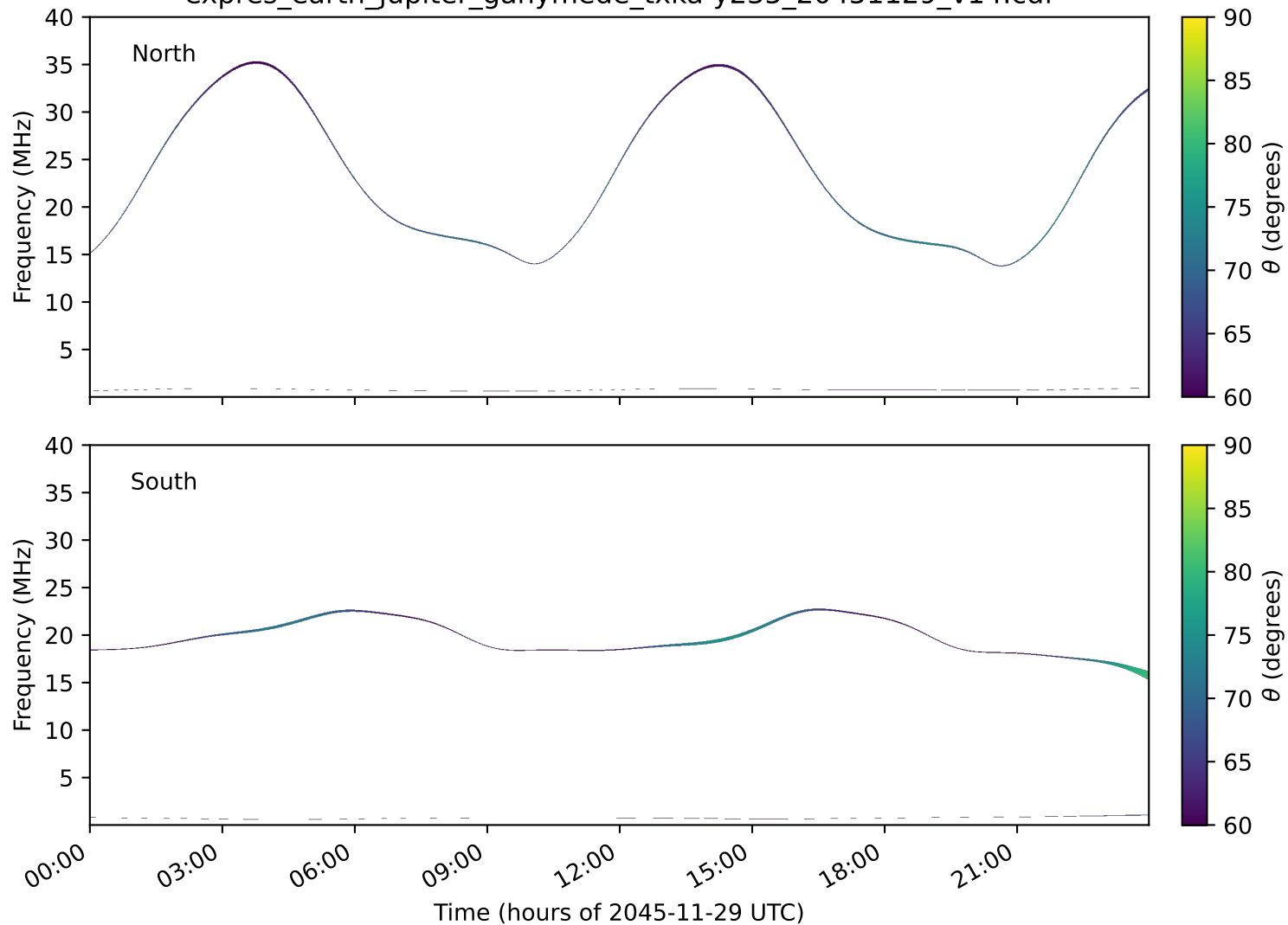
expres_earth_jupiter_ganymede_txka-y235_20451129_v14.cdf
