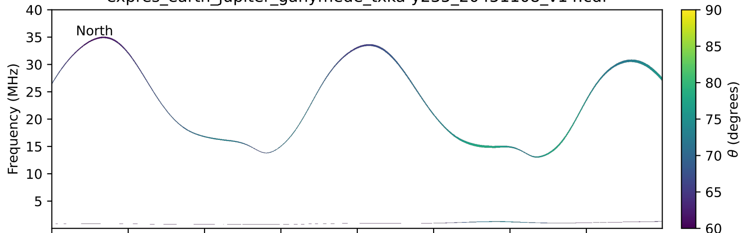
expres_earth_jupiter_ganymede_txka-y235_20451108_v14.cdf
