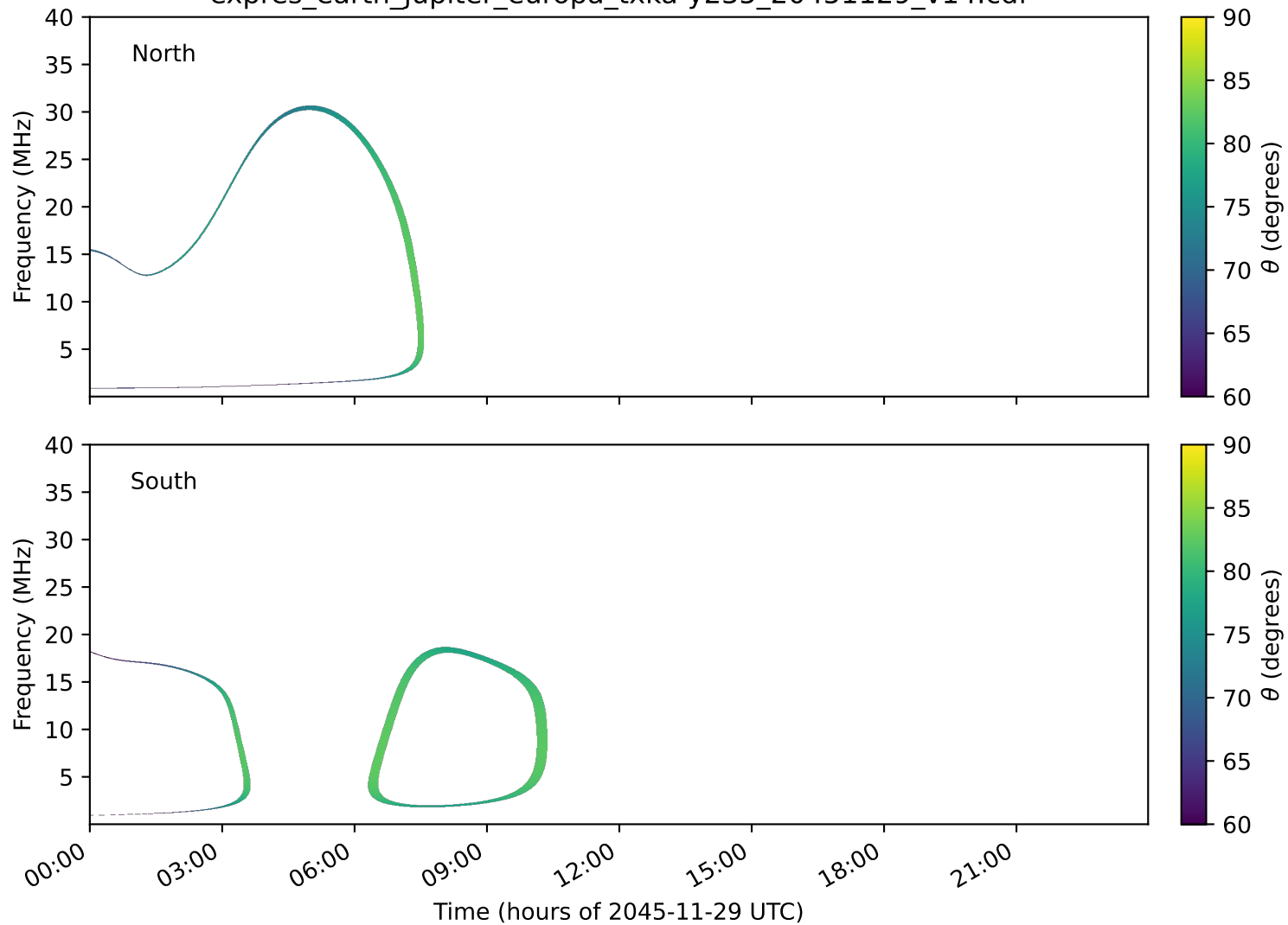
expres_earth_jupiter_europa_txka-y235_20451129_v14.cdf
