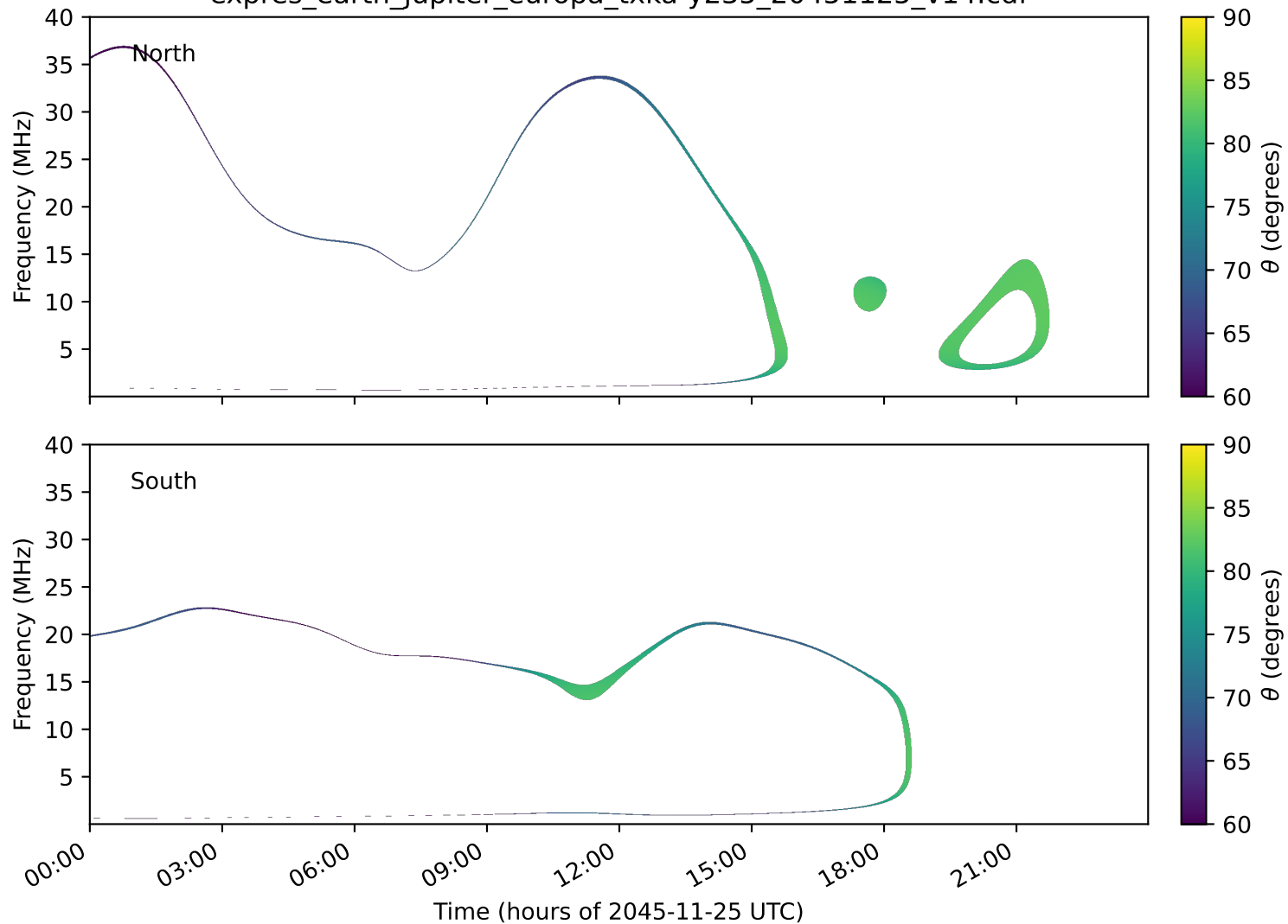
expres_earth_jupiter_europa_txka-y235_20451125_v14.cdf
