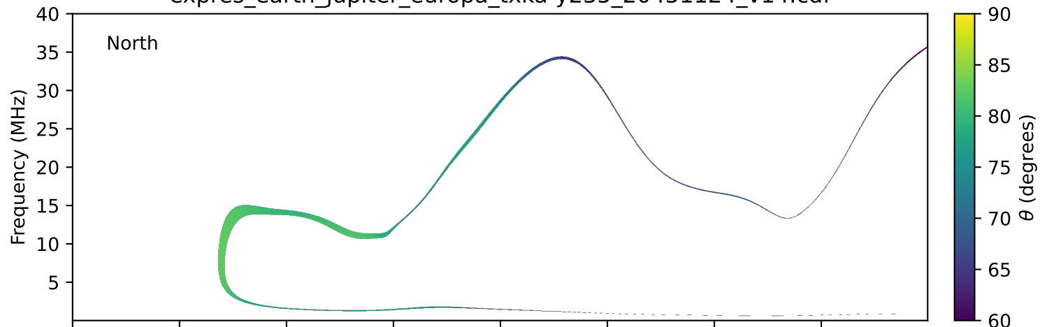
expres_earth_jupiter_europa_txka-y235_20451124_v14.cdf
