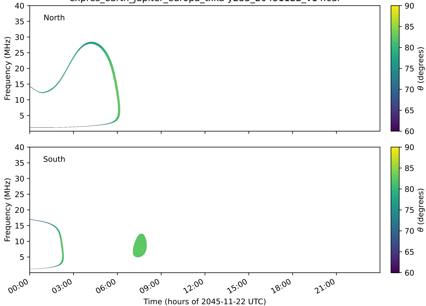
expres_earth_jupiter_europa_txka-y235_20451122_v14.cdf
