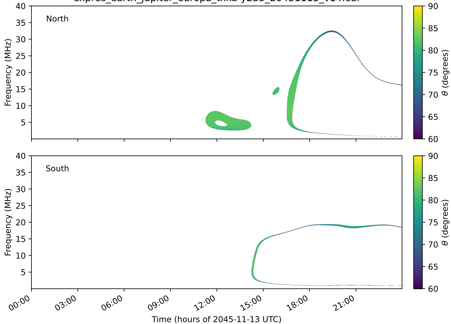
expres_earth_jupiter_europa_txka-y235_20451113_v14.cdf
