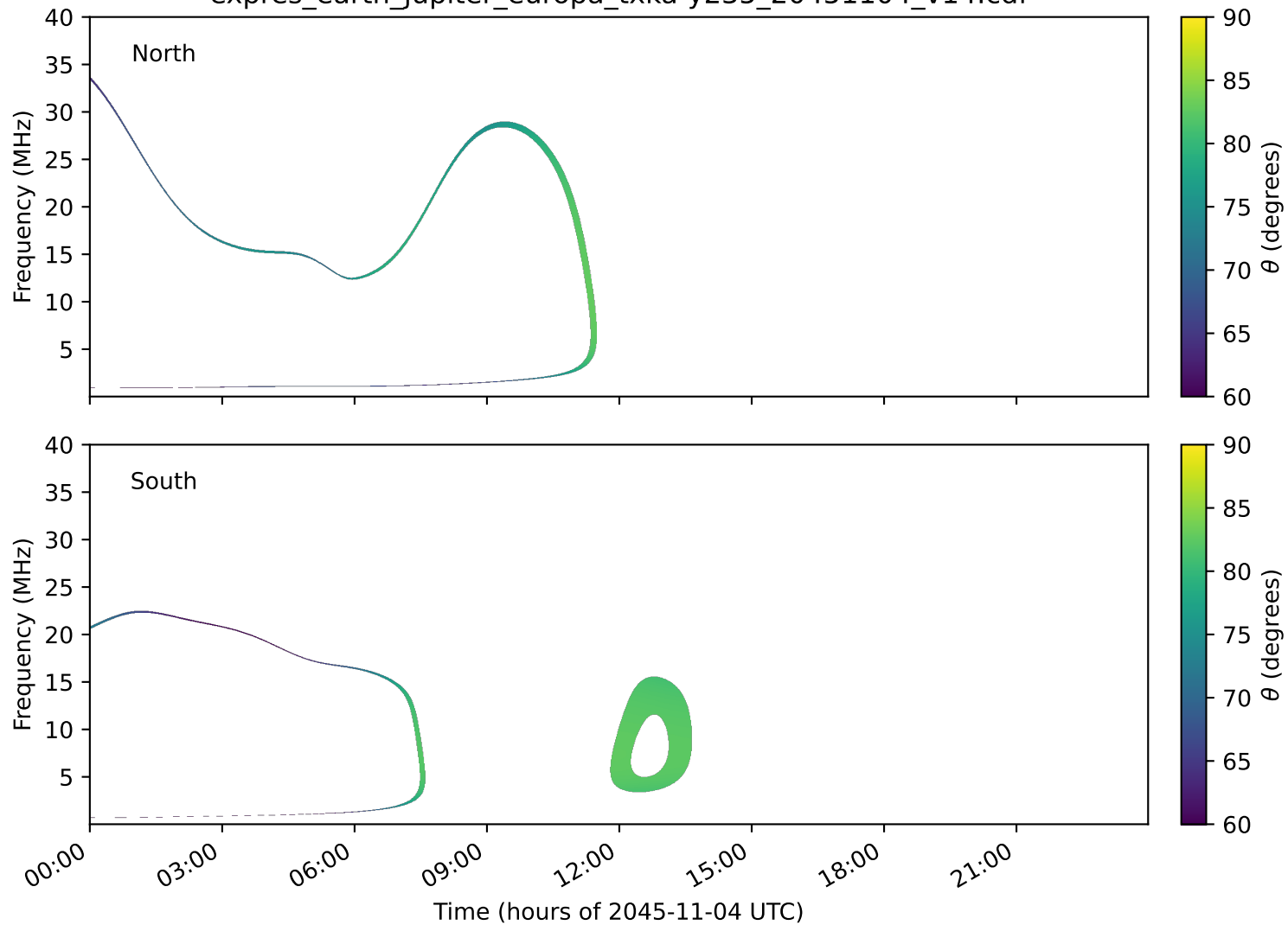
expres_earth_jupiter_europa_txka-y235_20451104_v14.cdf
