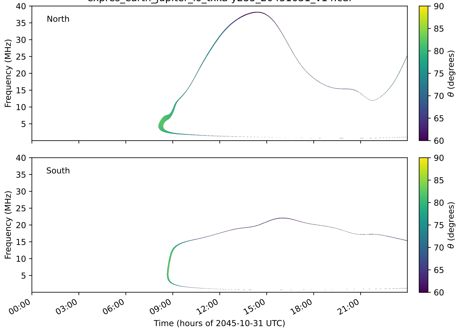
expres_earth_jupiter_io_txka-y235_20451031_v14.cdf
