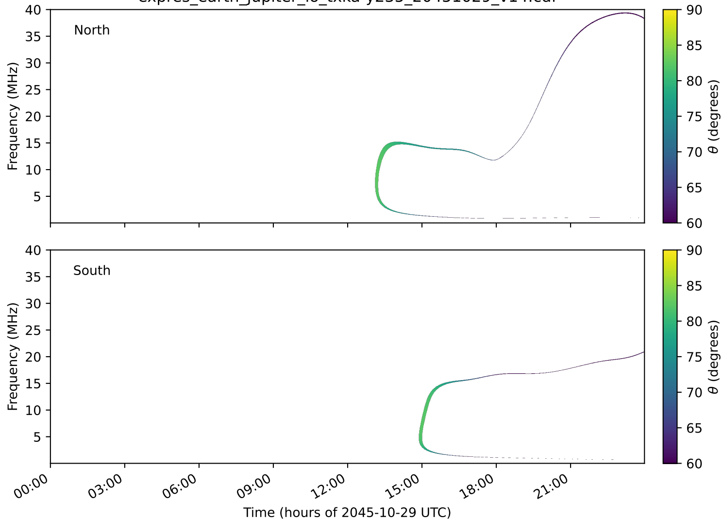
expres_earth_jupiter_io_txka-y235_20451029_v14.cdf
