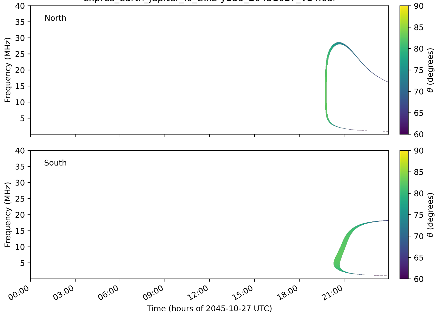
expres_earth_jupiter_io_txka-y235_20451027_v14.cdf
