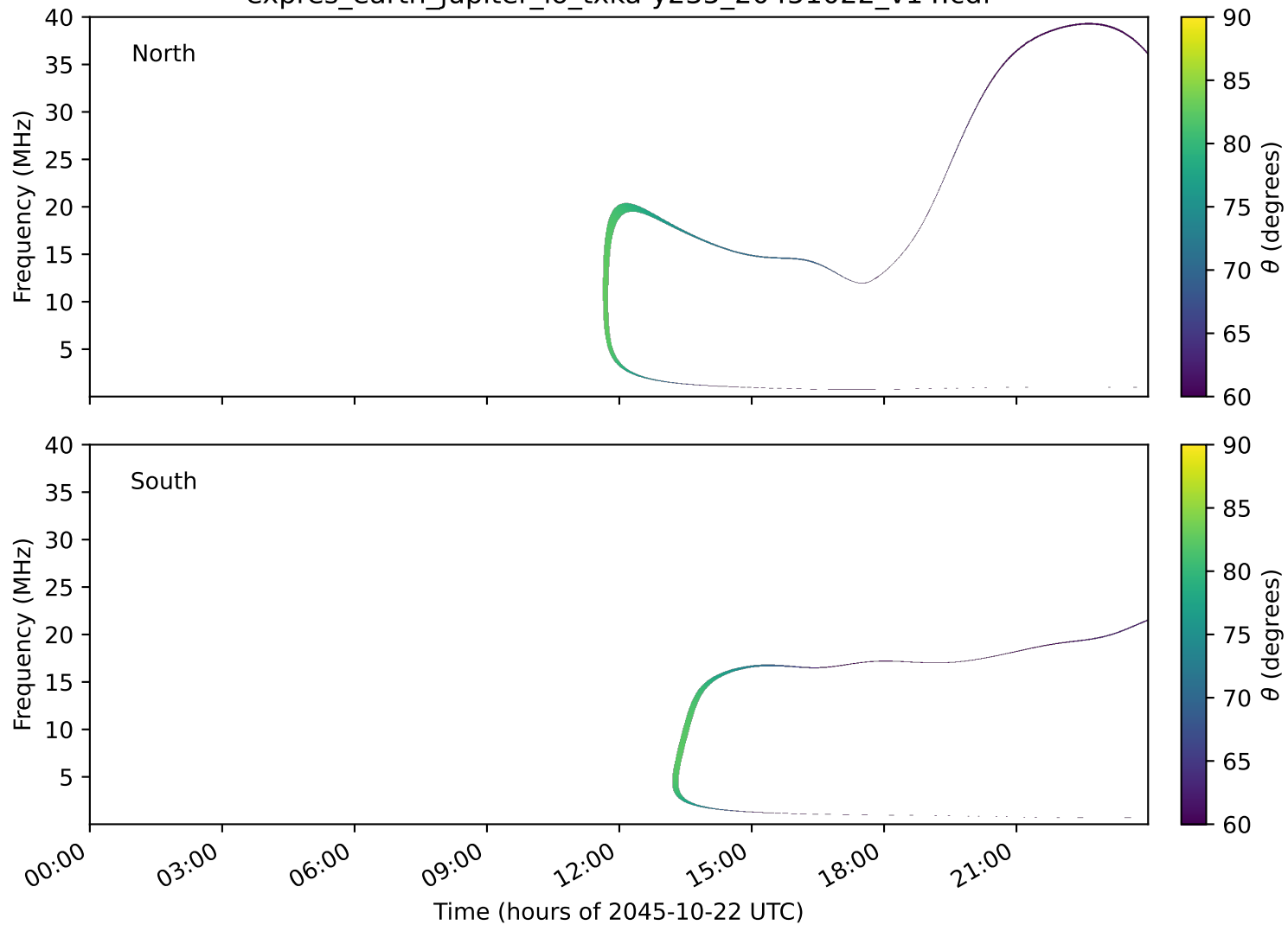
expres_earth_jupiter_io_txka-y235_20451022_v14.cdf
