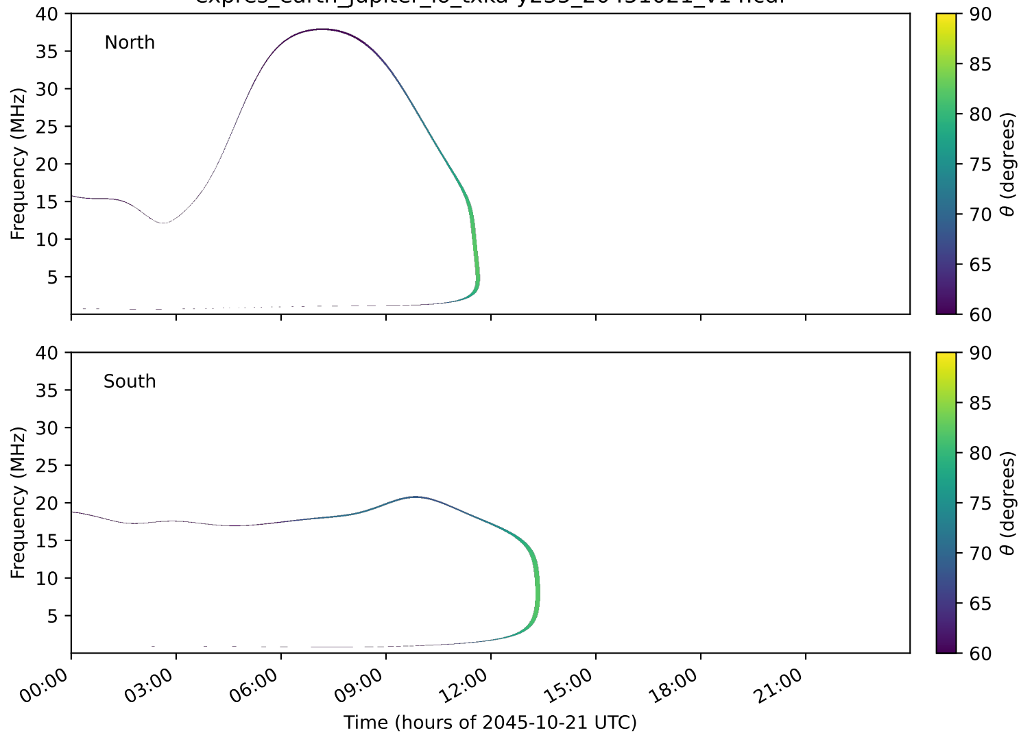
expres_earth_jupiter_io_txka-y235_20451021_v14.cdf
