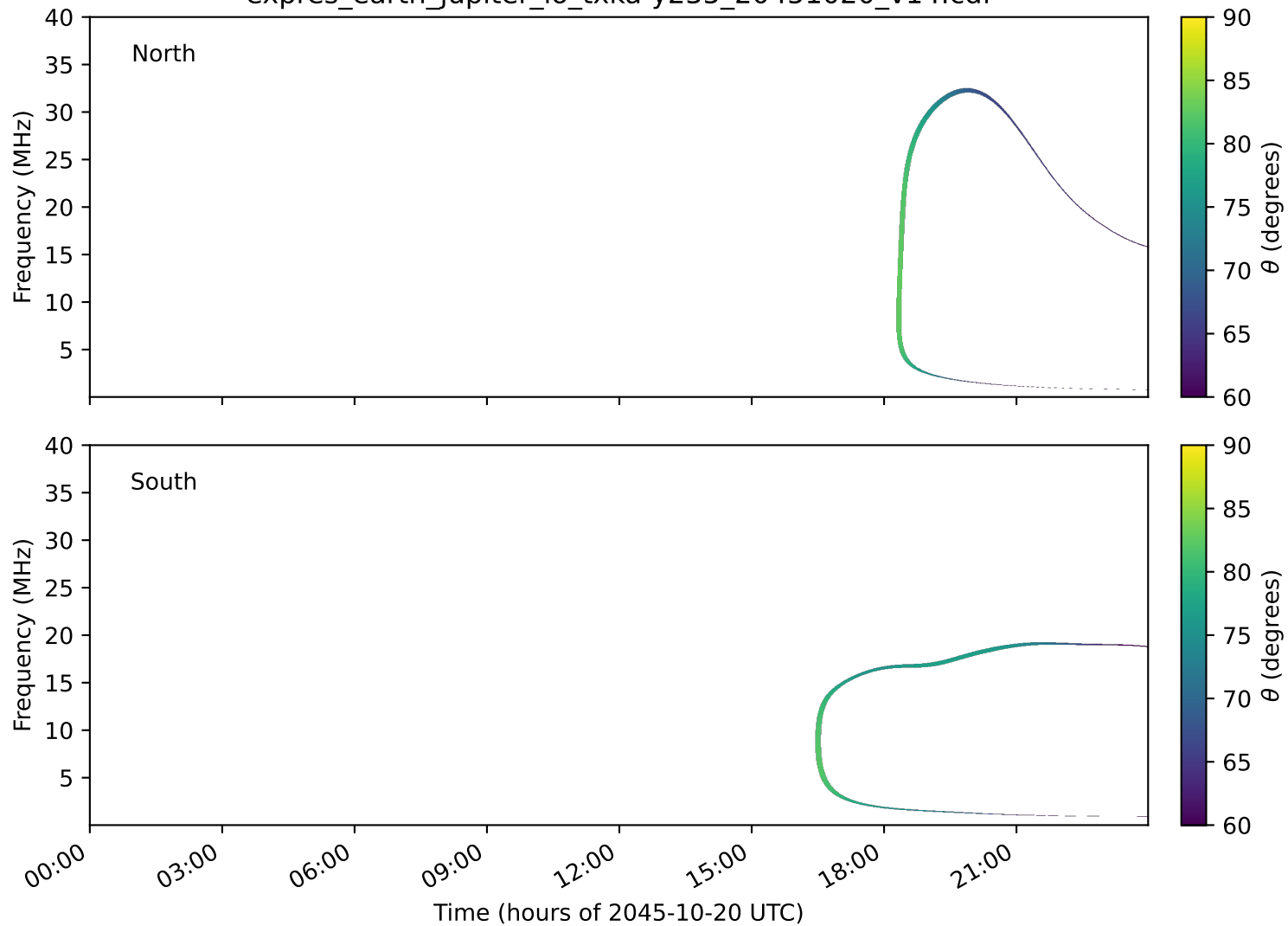
expres_earth_jupiter_io_txka-y235_20451020_v14.cdf
