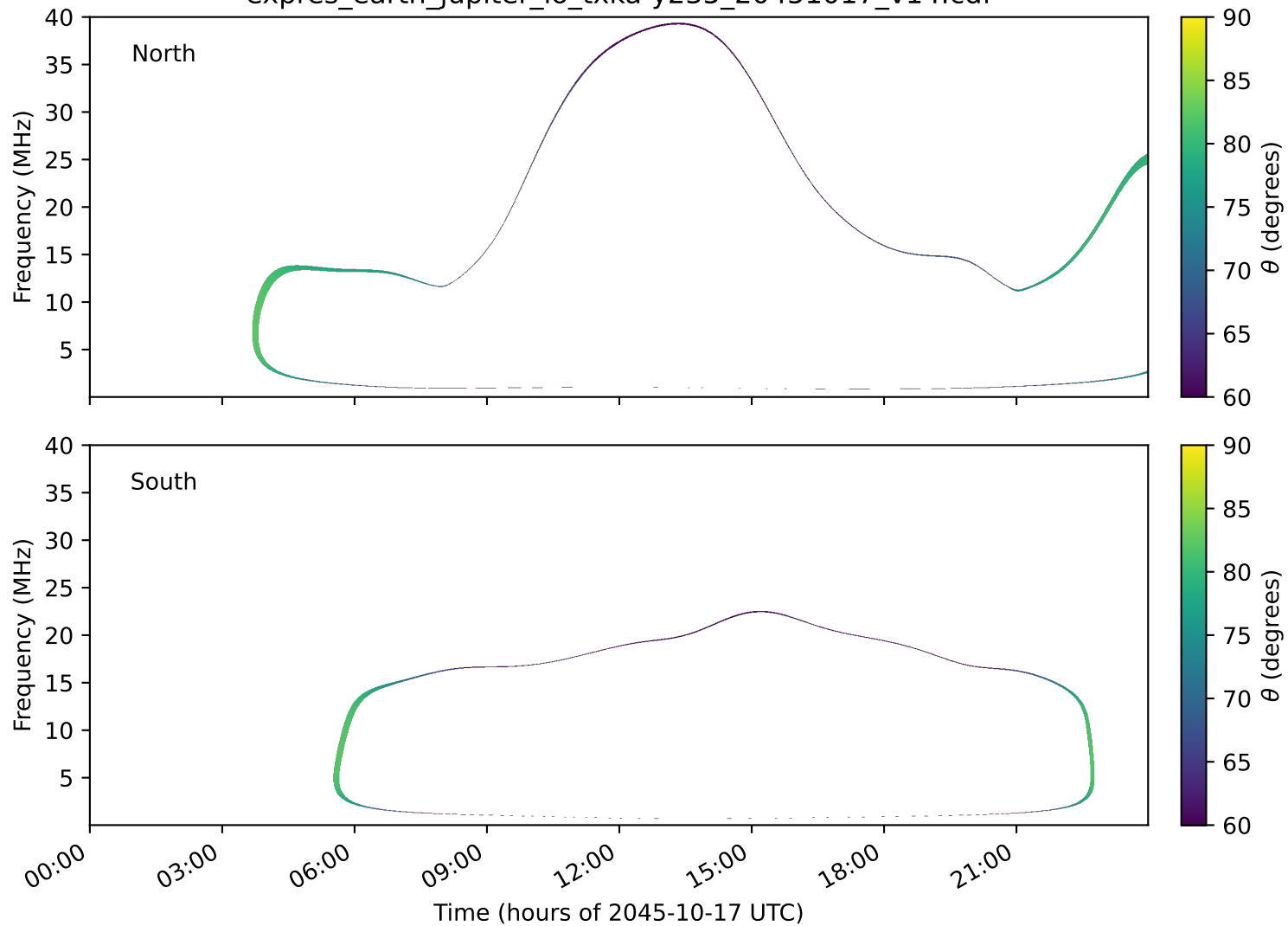
expres_earth_jupiter_io_txka-y235_20451017_v14.cdf
