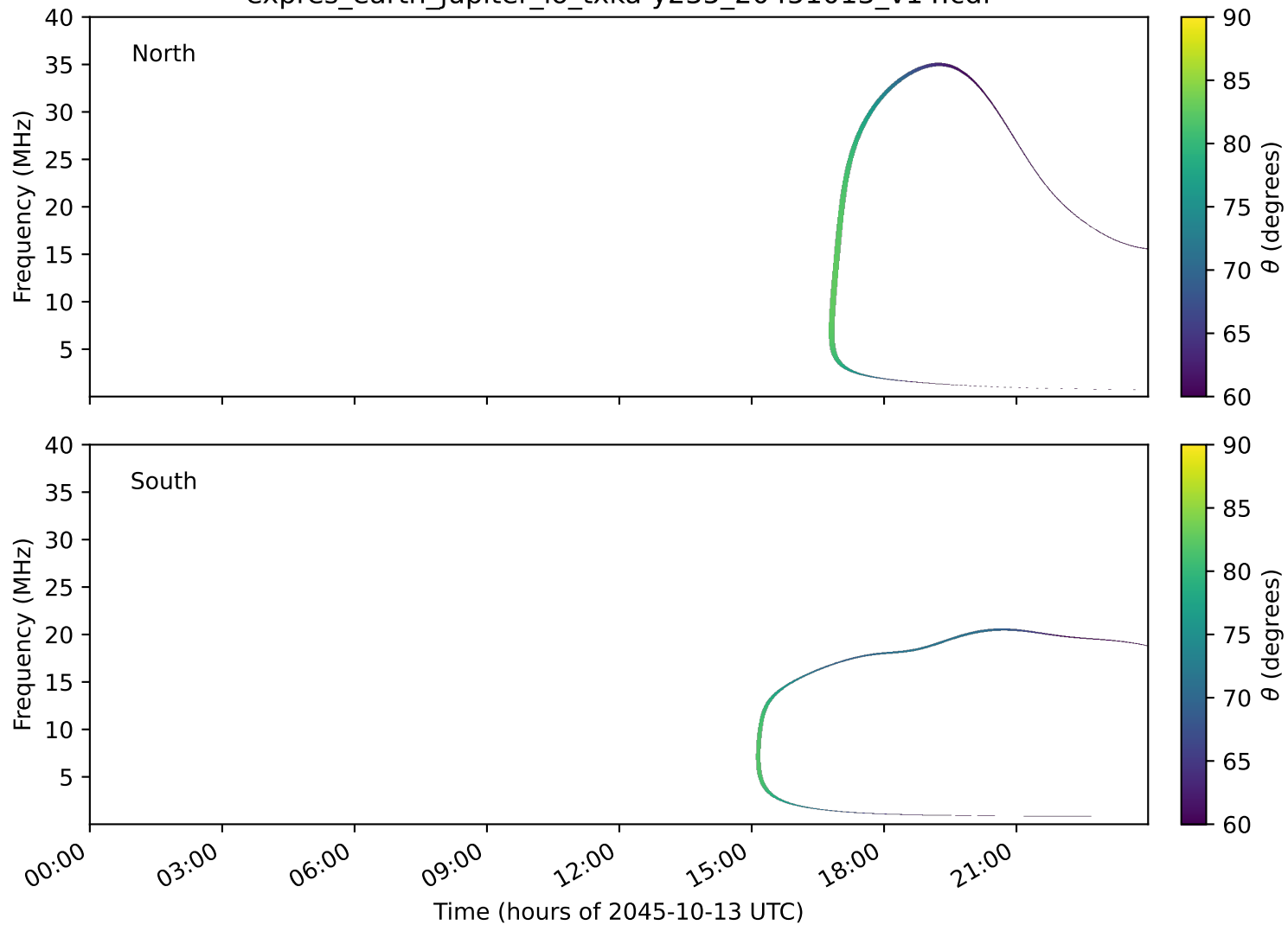
expres_earth_jupiter_io_txka-y235_20451013_v14.cdf
