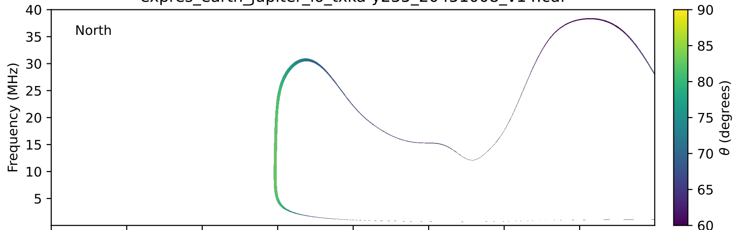
expres_earth_jupiter_io_txka-y235_20451008_v14.cdf
