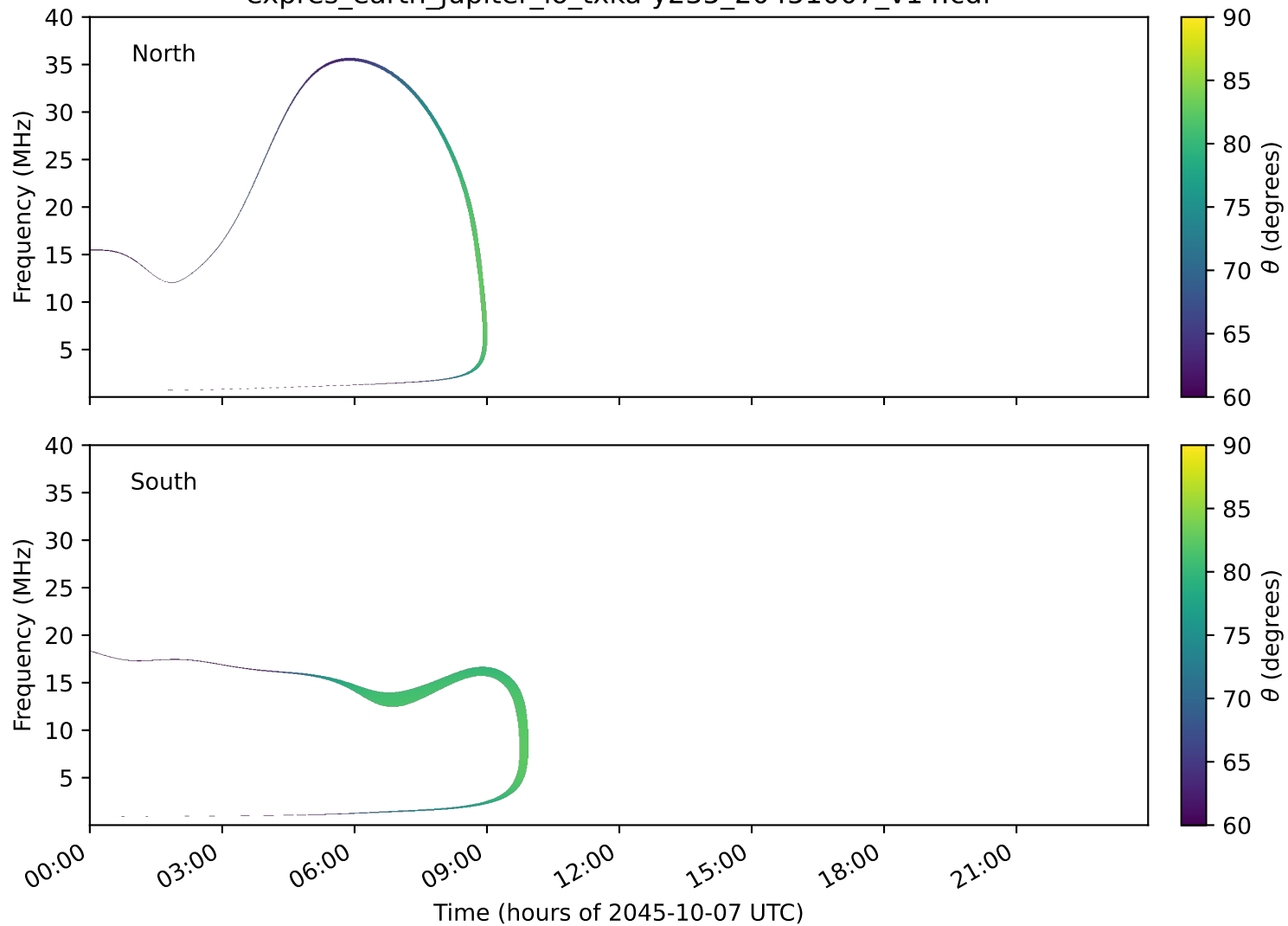
expres_earth_jupiter_io_txka-y235_20451007_v14.cdf
