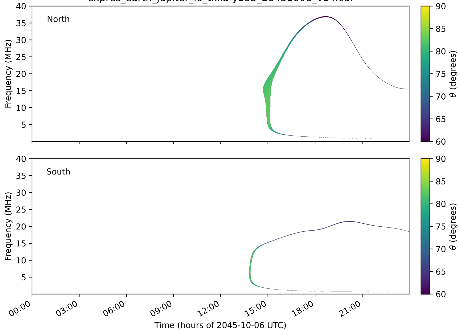
expres_earth_jupiter_io_txka-y235_20451006_v14.cdf
