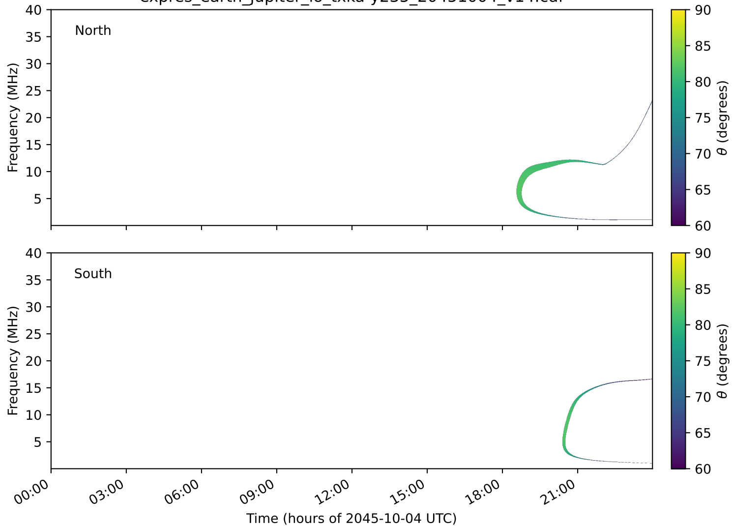
expres_earth_jupiter_io_txka-y235_20451004_v14.cdf
