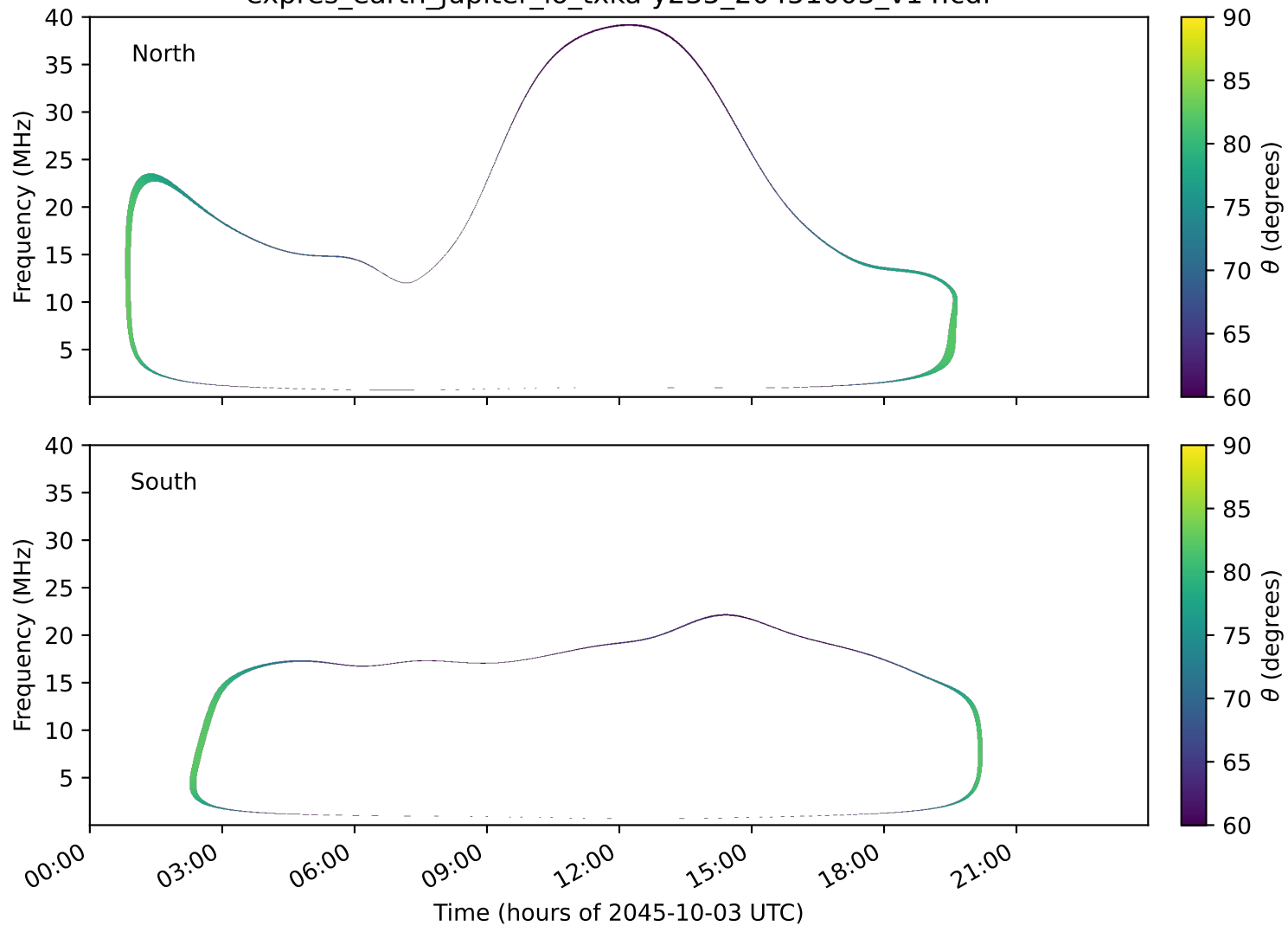
expres_earth_jupiter_io_txka-y235_20451003_v14.cdf
