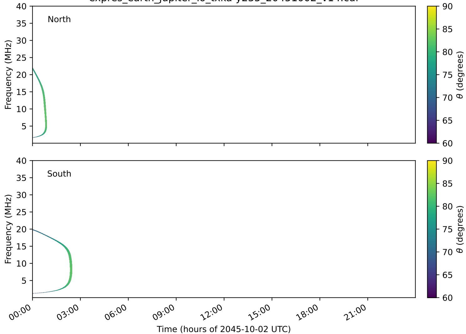
expres_earth_jupiter_io_txka-y235_20451002_v14.cdf
