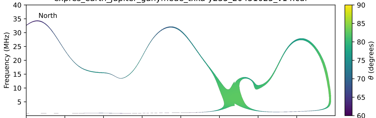
expres_earth_jupiter_ganymede_txka-y235_20451025_v14.cdf
