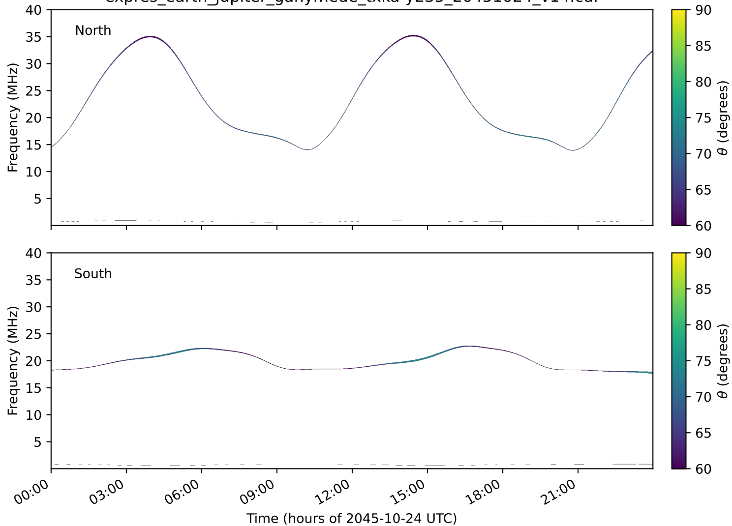
expres_earth_jupiter_ganymede_txka-y235_20451024_v14.cdf
