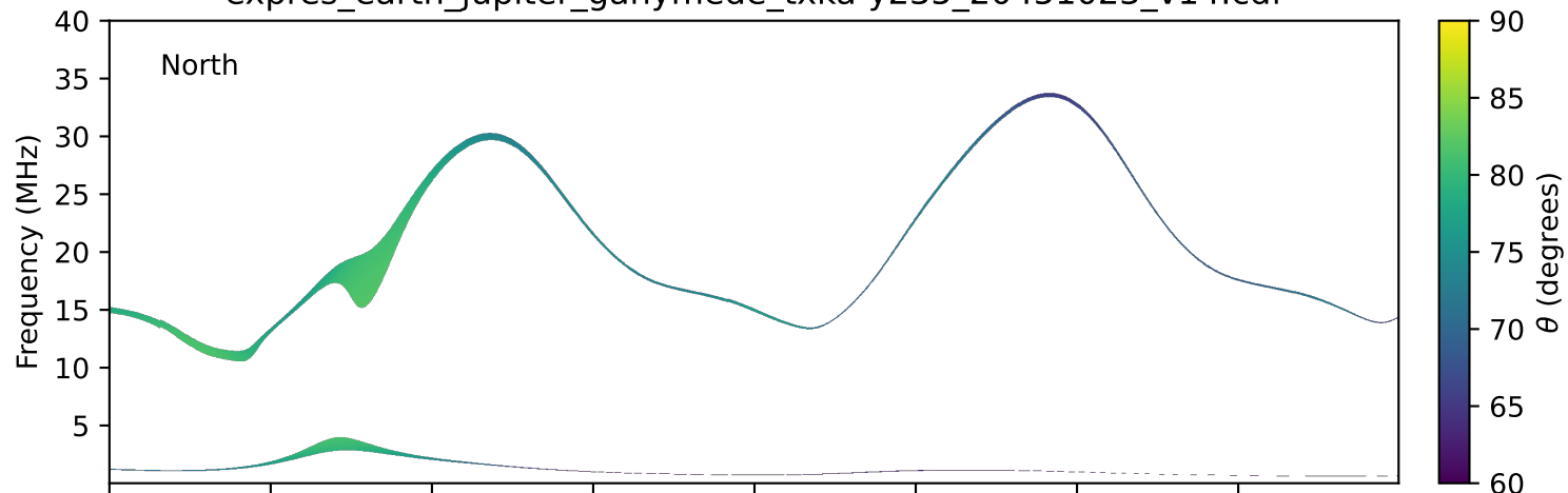
expres_earth_jupiter_ganymede_txka-y235_20451023_v14.cdf
