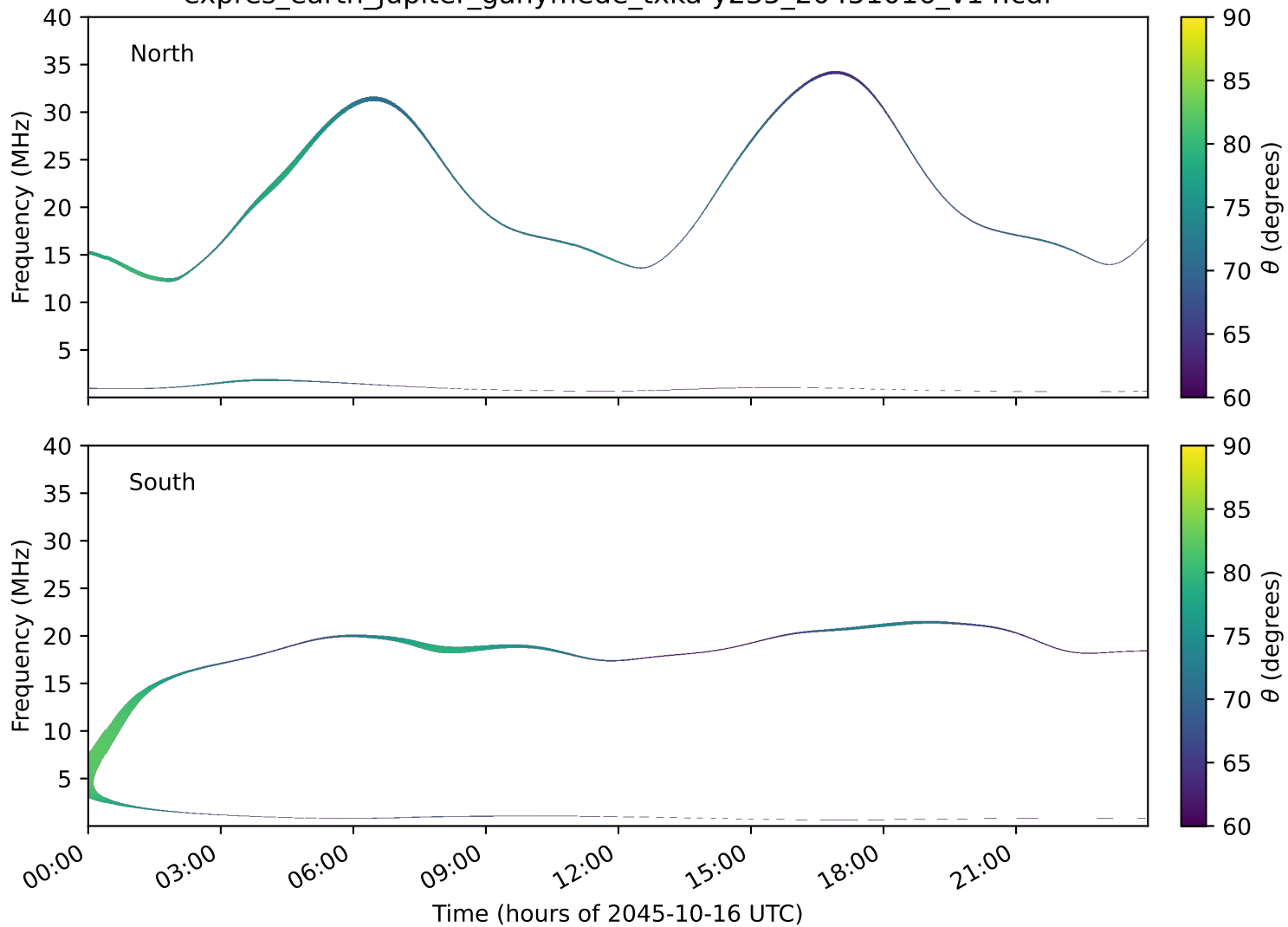
expres_earth_jupiter_ganymede_txka-y235_20451016_v14.cdf
