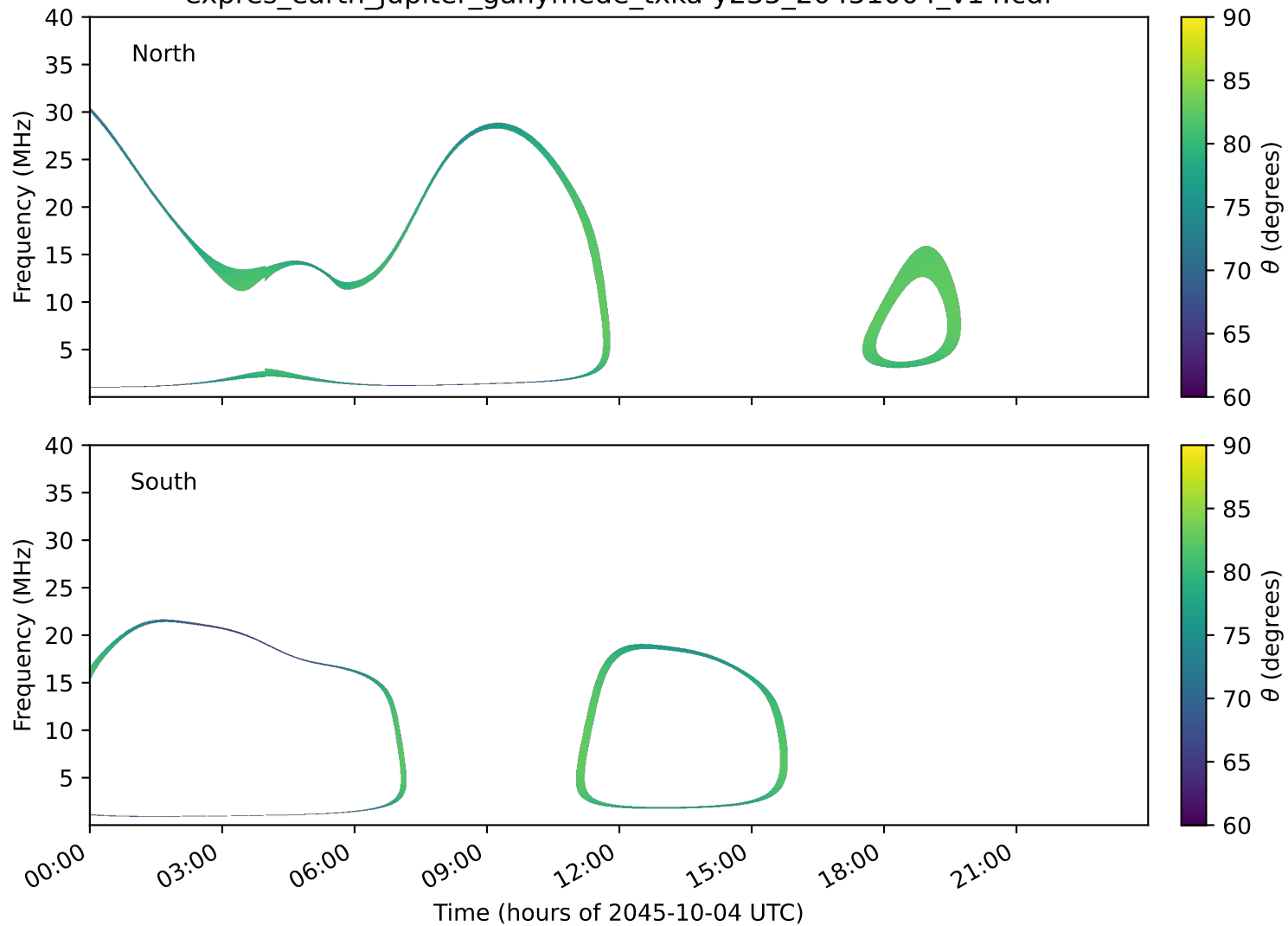
expres_earth_jupiter_ganymede_txka-y235_20451004_v14.cdf
