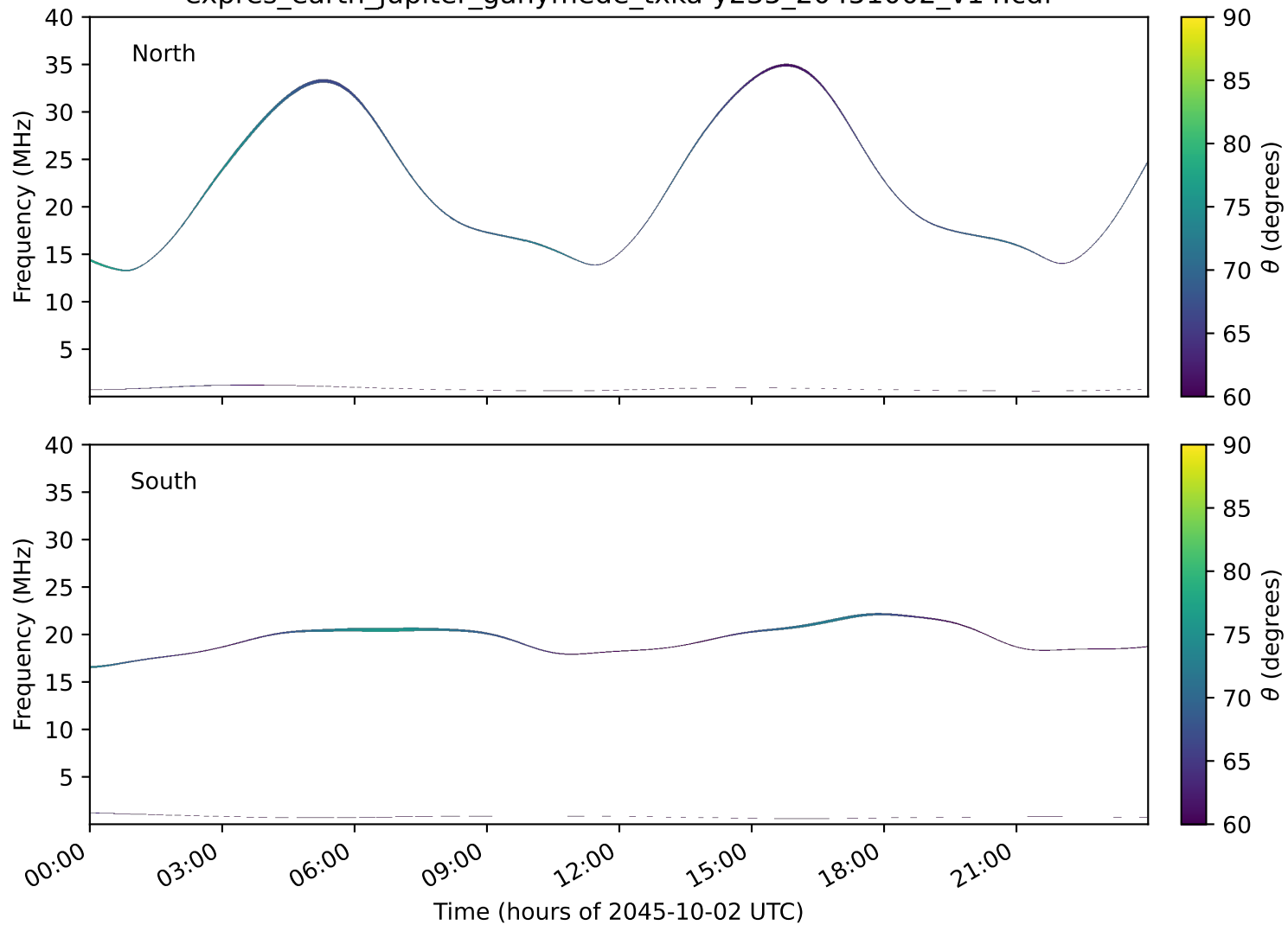
expres_earth_jupiter_ganymede_txka-y235_20451002_v14.cdf
