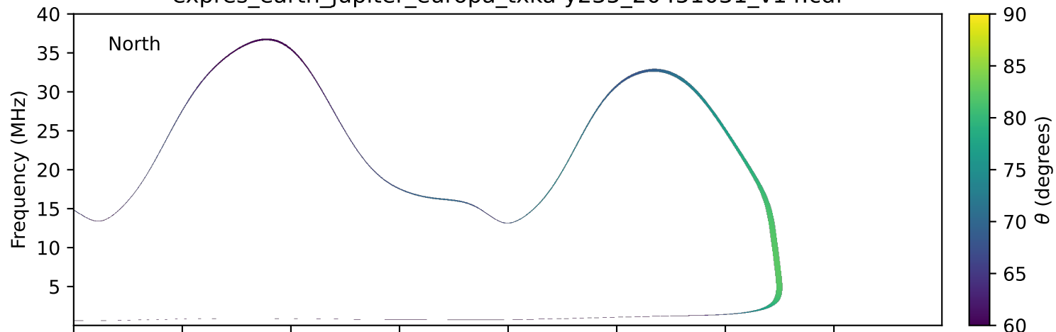
expres_earth_jupiter_europa_txka-y235_20451031_v14.cdf
