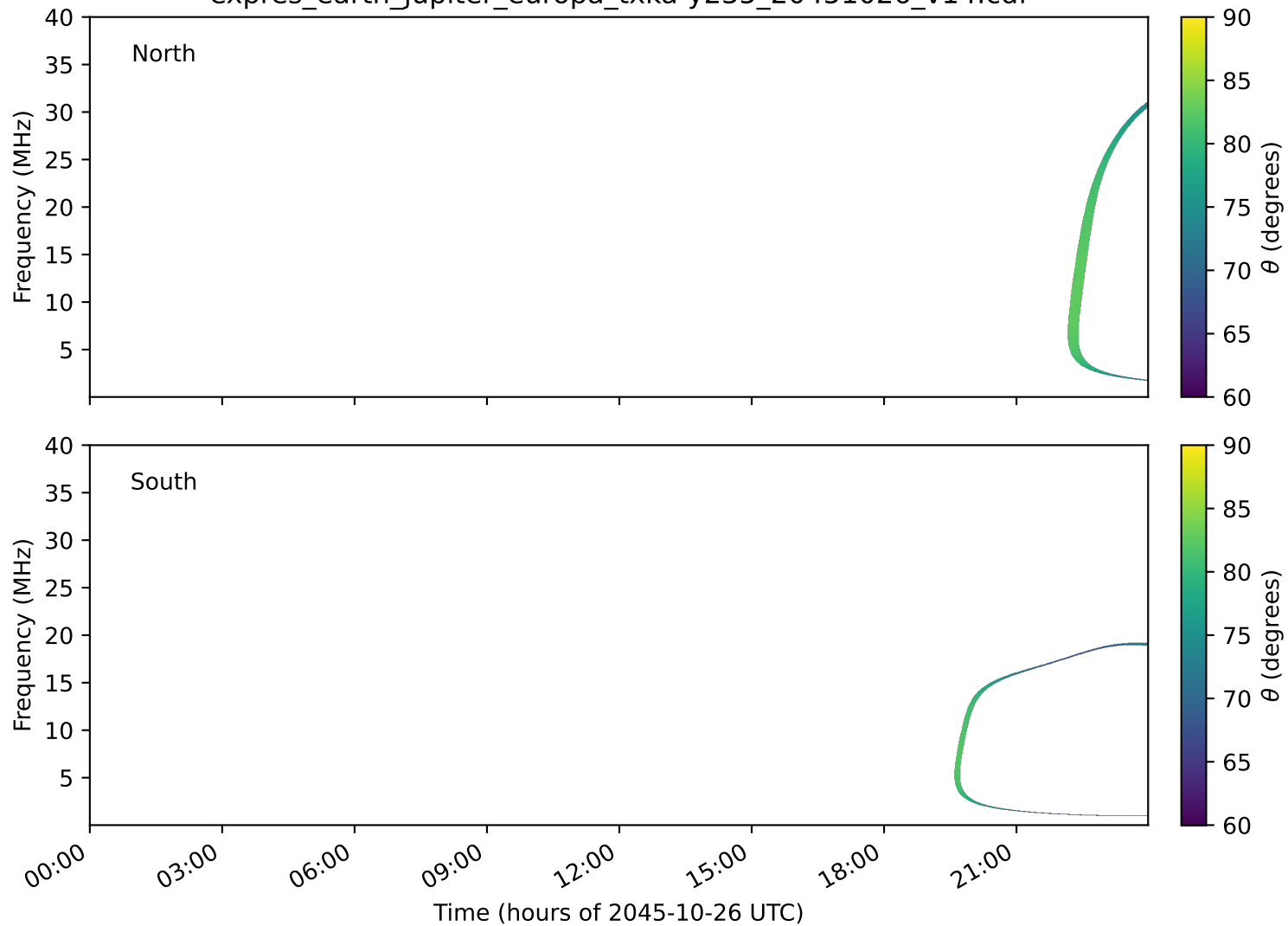
expres_earth_jupiter_europa_txka-y235_20451026_v14.cdf
