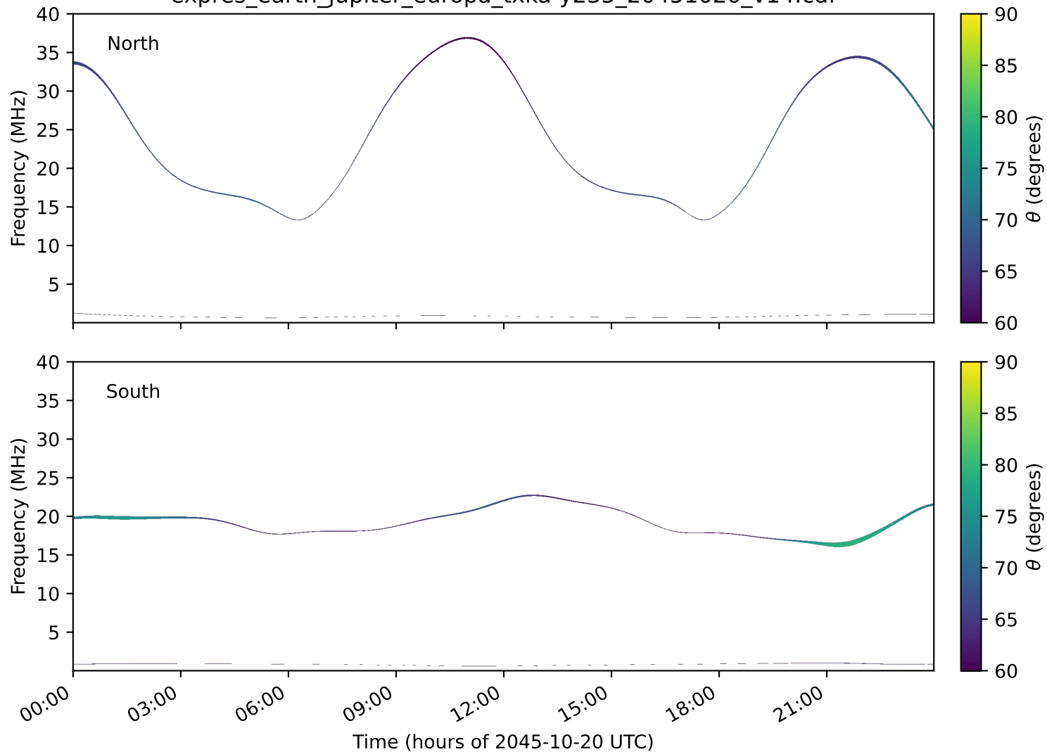
expres_earth_jupiter_europa_txka-y235_20451020_v14.cdf
