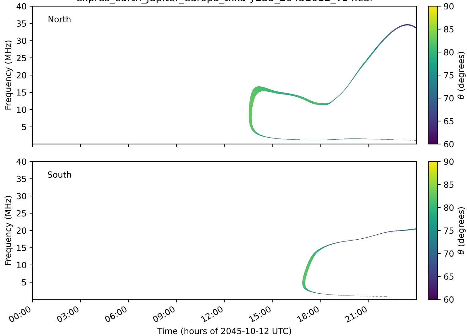
expres_earth_jupiter_europa_txka-y235_20451012_v14.cdf
