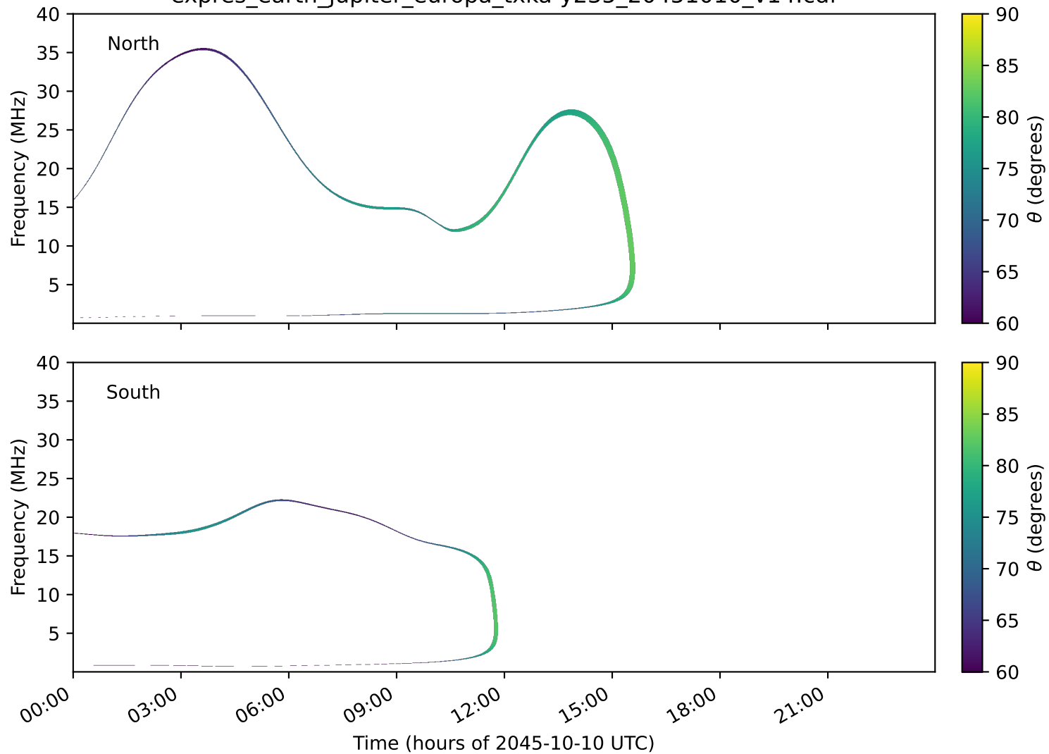
expres_earth_jupiter_europa_txka-y235_20451010_v14.cdf
