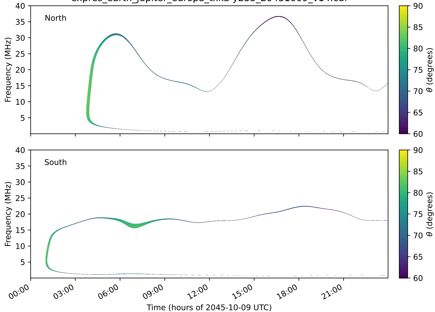
expres_earth_jupiter_europa_txka-y235_20451009_v14.cdf
