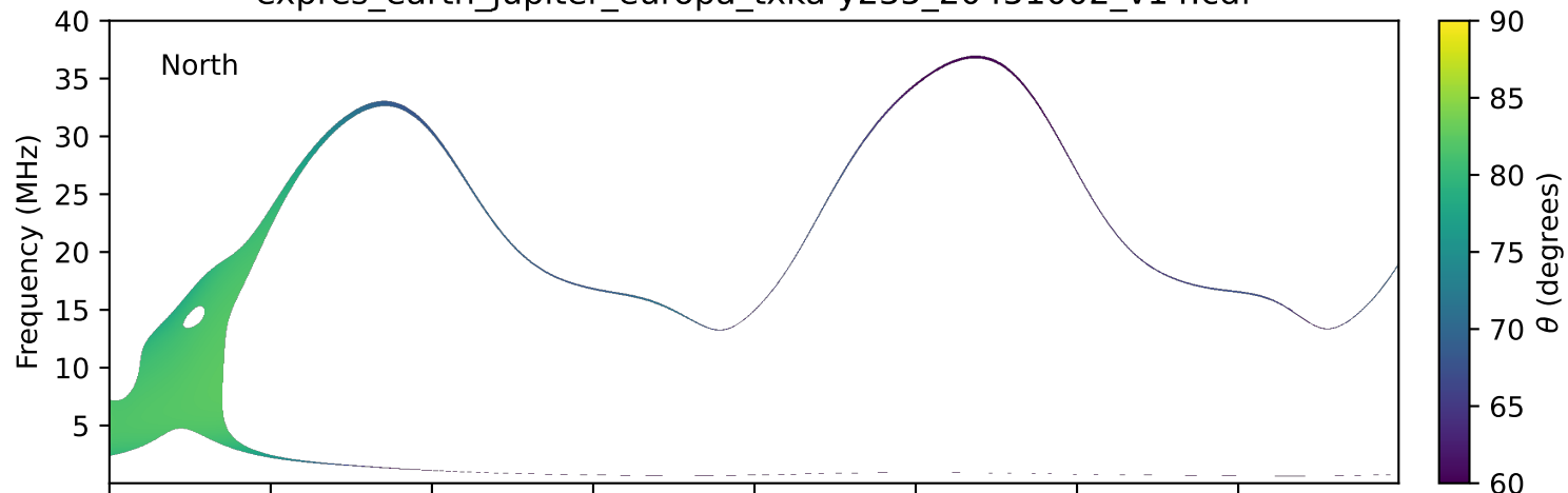
expres_earth_jupiter_europa_txka-y235_20451002_v14.cdf
