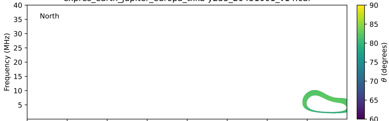
expres_earth_jupiter_europa_txka-y235_20451001_v14.cdf
