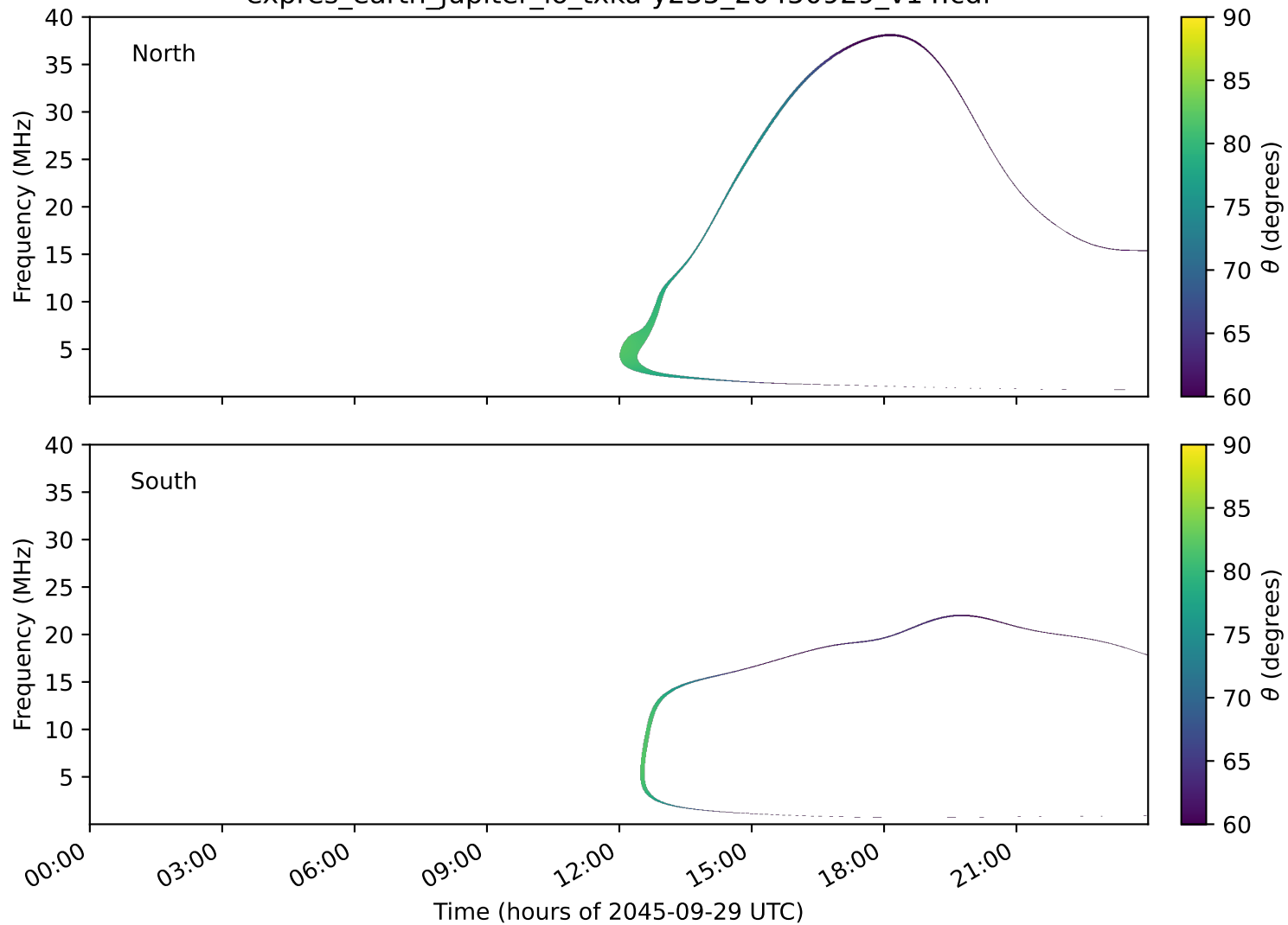
expres_earth_jupiter_io_txka-y235_20450929_v14.cdf
