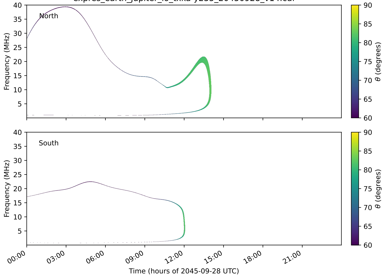
expres_earth_jupiter_io_txka-y235_20450928_v14.cdf
